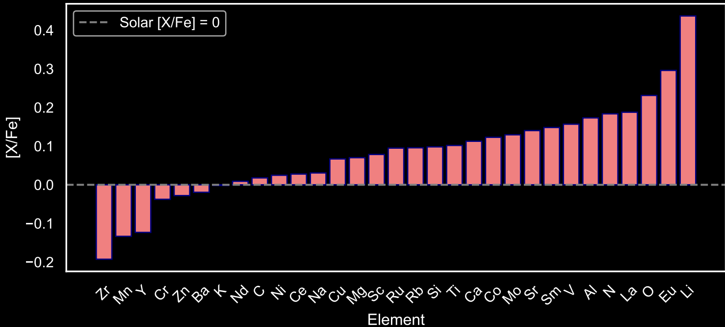
Abundance Pattern for GALAH Star Field [87] (N=124)
