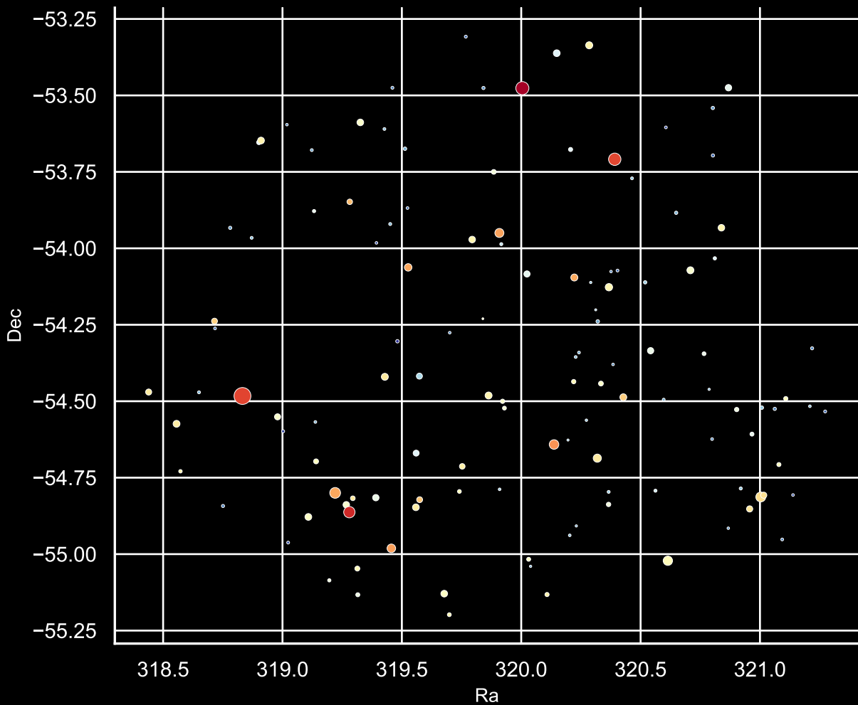
Field [87] Ra [319.96] Dec [-54.36] Stars: 124
