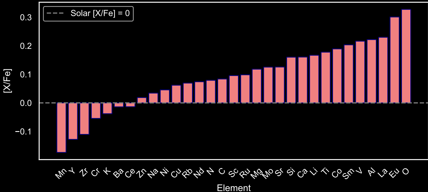
Abundance Pattern for GALAH Red Giants: Star Field [87] (N=64)
