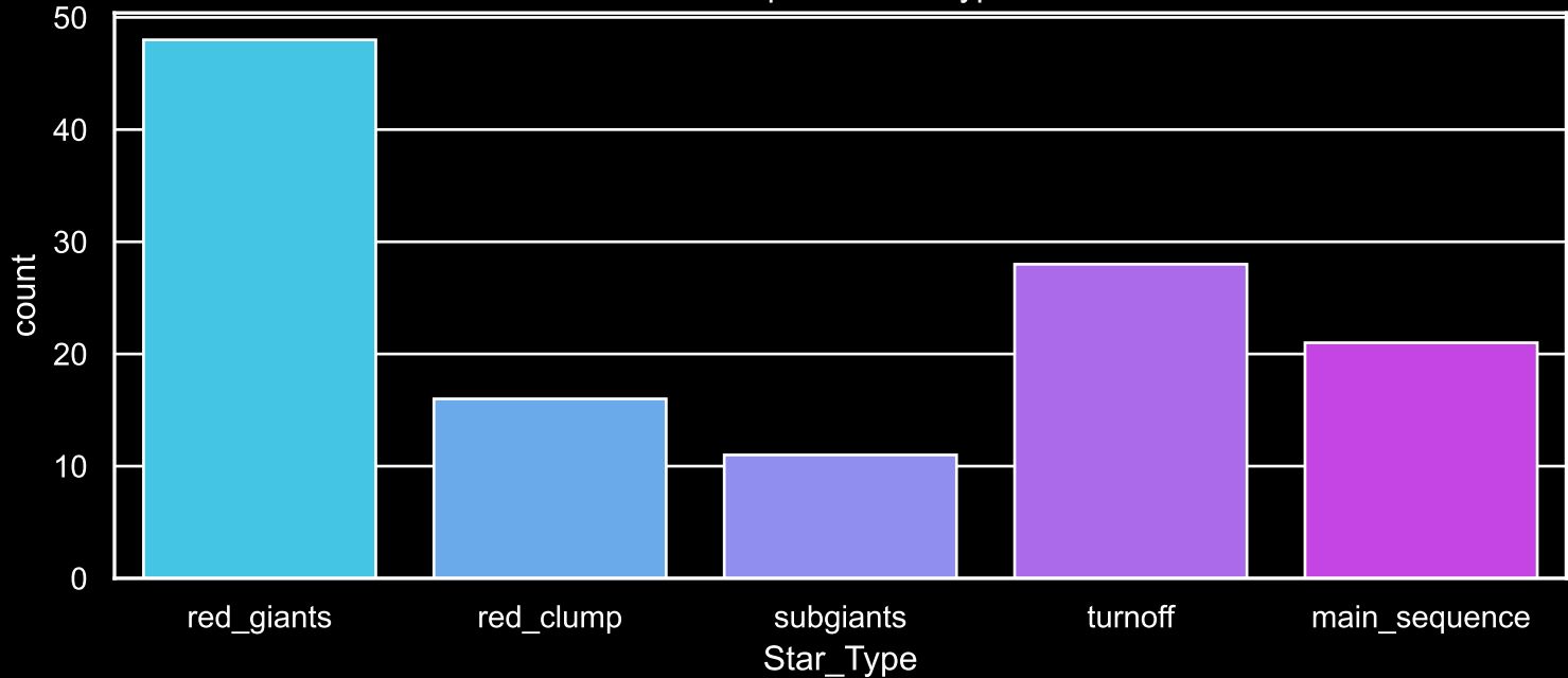
Field [87] Count plot of Star Type
