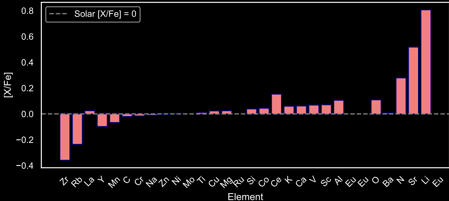
Abundance Pattern for GALAH Main Sequence Stars: Star Field [87] (N=21)
