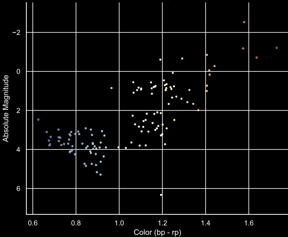
GALAH Hertzprung-Russel Diagram Field [87] Ra [319.96] Dec [-54.36]
